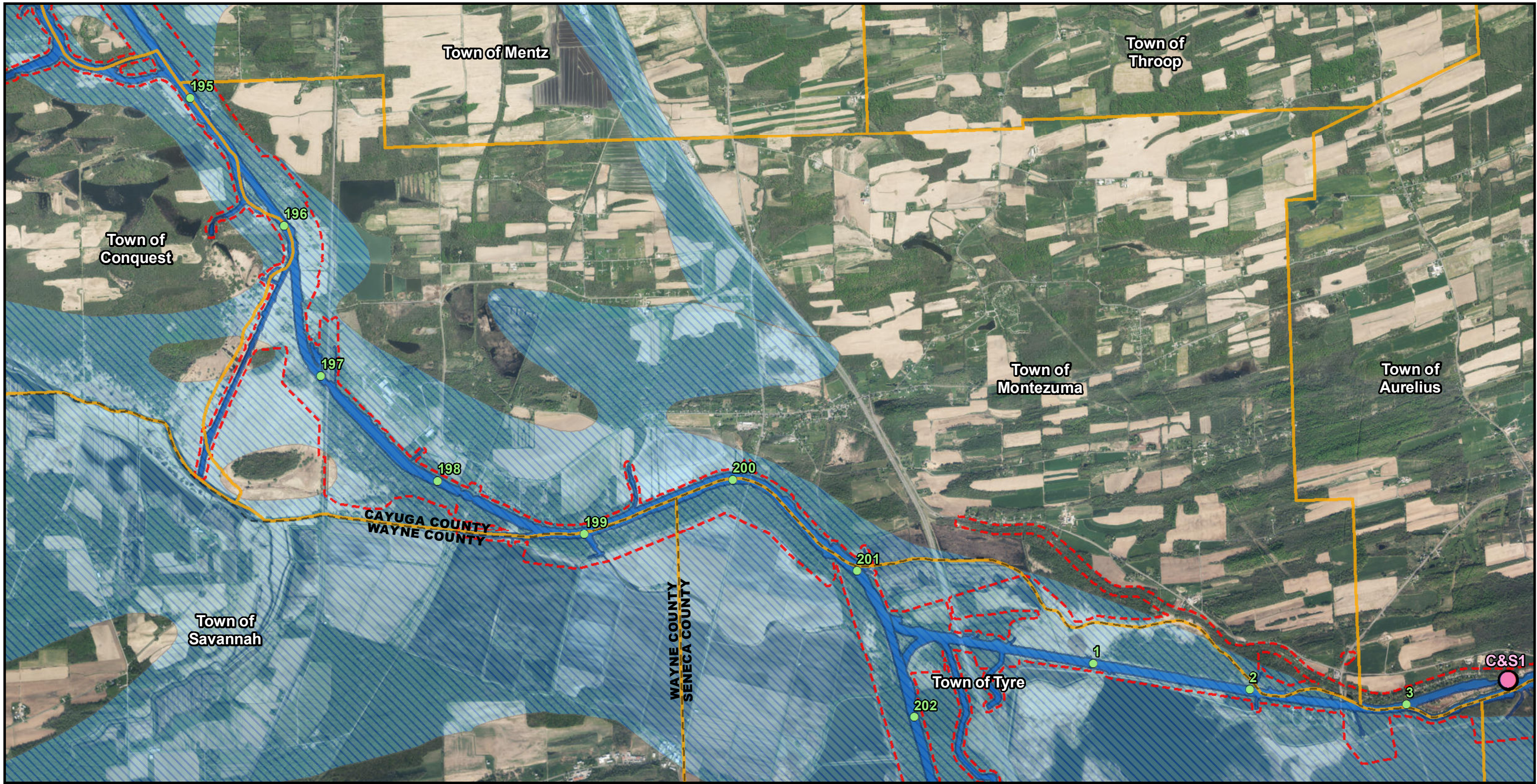
Figure 84F: Aquifers
